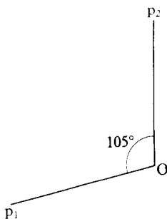
9.20 The water molecule. The bond angle with no hybridisation would be 90^\circ .
